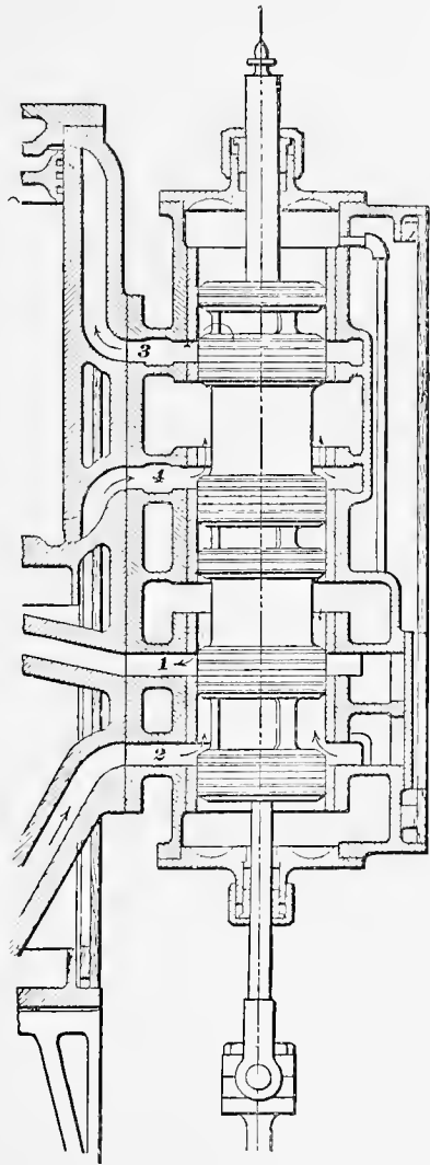
FIG. 3.—CANFIELD'S BALANCE VALVE.
